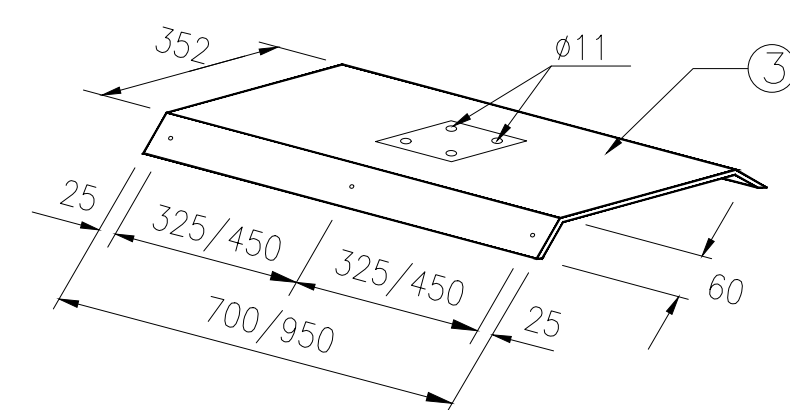
DETAIL 'D'
